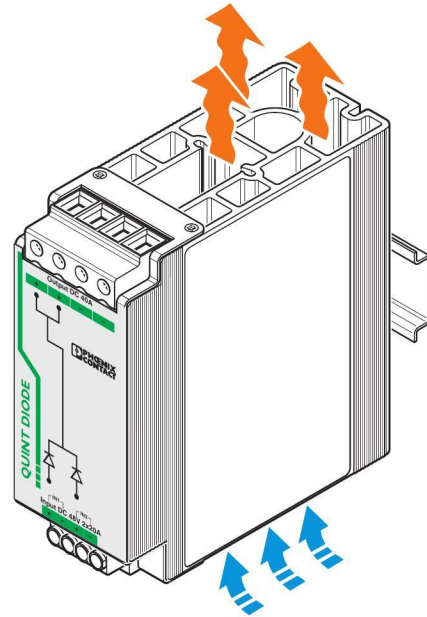
Figure 2 Convection
